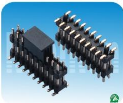
01.5系列: 2.54mm双排针,双塑,SMT (可带定位柱及夹持盖) Spec:2.54mm Board Spacer,Dual Row,SMT With Locating Peg or CAP Positions:2*2~2*40 Plastics Height:2.54mm
