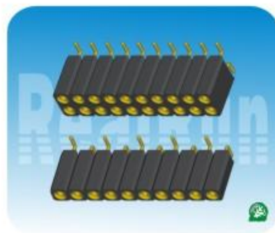
02.B系列:2.54mm 圆孔 SMT Spec:2.54mm Pitch Machine Pin Socket Single/Dual Row SMT Plastics Height:1.9/3.0/4.2/7.0 Positions:1*2~1*40/2*2~2*40
