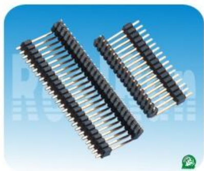
01.3系列: 1.27mm单排,双塑,90度 塑高1.0/1.7/2.0/2.54mm Spec:1.27mm Dual Plastics,Single Row,Right Angle Positions:1*2~1*50 Plastics Height:1.0/1.7/2.0/2.54mm
