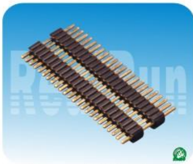
01.3系列: 1.27mm单排,双塑,180度 塑高1.0/1.7/2.0/2.54mm Spec:1.27mm Board Spacer,Single Row,Straight Positions:1*2~1*50 Plastics Height:1.0/1.7/2.0/2.54mm
