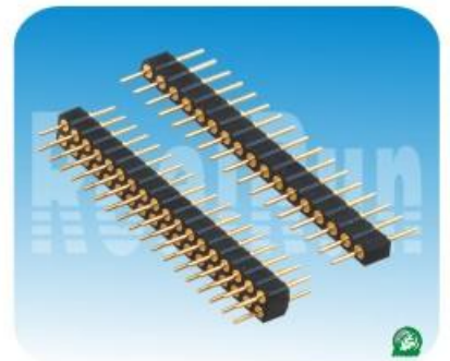
01.8系列:2.0mm 圆针 单/双排 180度 Spec:2.0mm Pitch Machine Pin Adapters Single/Dual Row Straight Plastics Height:2.8 Positions:1*2~1*40/2*2~2*40
