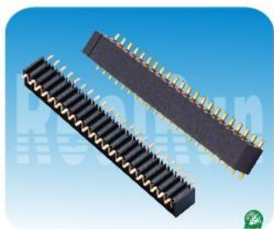
02.4系列: 2.0mm双排母,90度,双侧插,SMT Spec:2.0mm Female Header,Dual Row,Side Entry,SMT Positions:2*2~2*40 Plastics Height:4.9mm
