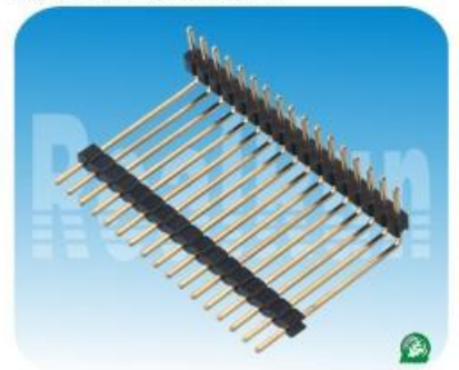
01.4 系列: 2.0mm单排针,双塑,90度 R2TYPE Spec:2.0mm Dual Plastics,Single Row, Right Angle,Type 2 Positions:1*2~1*40 Plastics Height:2.0mm
