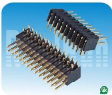
01.5系列: 2.54mm双排针,180度 Spec:2.54mm Pin Header,Dual Row,Straight Positions:2*3~2*40 Plastics Height:7.4mm
