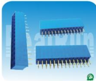
02.5系列 2.54mm双排母,180° Y型端子、蓝色 Spec:2.54mm Female Header,Dual Row, Straight,Blue Positions:2*2~2*40 Plastics Height:8.5mm Y-Type Terminal
