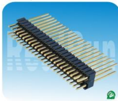
01.3系列: 1.27*2.54mm双排针,180度 Spec:1.27mm Pin Header,Dual Row,Straight Positions:2*2~2*50 Plastics Height:1.7/2.54mm
