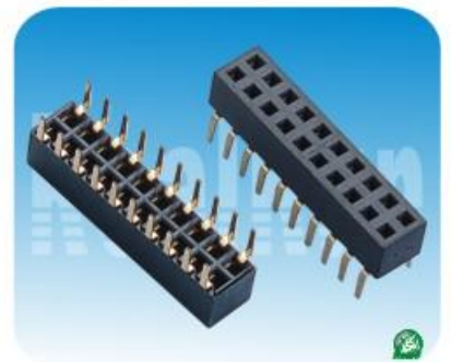
02.4系列: 2.0mm双排母,180度 5.0/6.0mm蜈蚣脚 Spec:2.0mm Female Header,Dual Row,Bottom Entry Positions:2*2~2*40 Plastics Height:4.3mm
