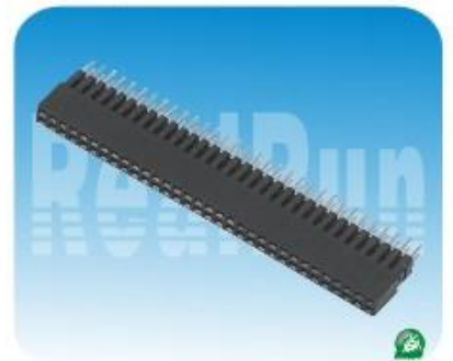
02.5系列: 2.54mm排母 双排 加高型 Spec:2.54mm Female Header Dual Row Plastics Height:8.5+2.5+2.5mm Positions:2*2~2*40
