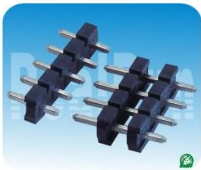
01.7系列:5.08mm 排针 单排 180度 单塑/多塑 Spec:5.08mm Pin Header Single Row Straight Positions:1*2~1*20 Plastics Height:2.54mm
