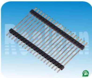
01.4 系列: 2.0mm单排针,双塑,180度 Spec:2.0mm Board Spacer,Single Row,Straight Positions:1*2~1*40 Plastics Height:1.5/2.0mm
