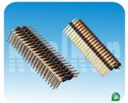
01.4 系列: 2.0mm双排针,双塑,90度 Spec:2.0mm Board Spacer,Dual Row,Right Angle Positions:2*2~2*40 Plastics Height:1.0/1.5/2.0mm
