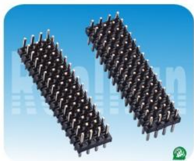
01.4 系列: 2.0mm四排针,180度 Spec:2.0mm Pin Header,Quad Row,Straight Positions:4*4~4*40 Plastics Height:1.5/2.0mm
