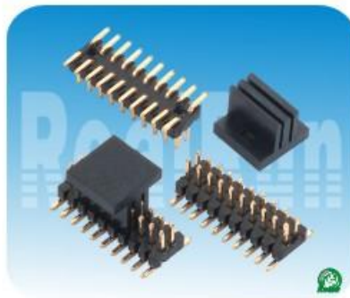
01.2系列: 1.0mm双排针,SMT (可带定位柱及夹持盖) Spec:1.0mm Pin Header,Dual Row,SMT With Locating Peg or CAP Positions:2*2~2*50 Plastics Height:1.0/1.5/2.0mm
