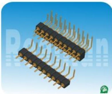
01.8系列:2.54mm 圆针 单/双排 90度 Spec:2.54mm Pitch Machine Pin Adapters Single/Dual Row Right Angle Plastics Height:1.9/3.0 Positions:1*2~1*40/2*2~2*40
