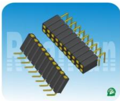
02.B系列:2.54mm 圆孔 单/双排 90度 Spec:2.54mm Pitch Machine Pin Socket Single/Dual Row Right Angle Plastics Height:1.9/3.0/4.2/7.0 Positions:1*2~1*40/2*2~2*40
