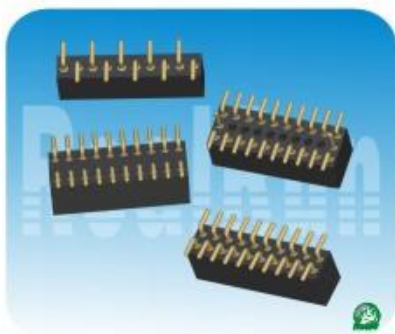
02.8系列:1.27mm 圆孔 单/双/三排 SMT Spec:1.27mm Pitch Machine Socket Single/Dual/Tripel Row SMT Plastics Height:4.0 Positions:1*2~1*50/2*2~2*50/3*2~3*50
