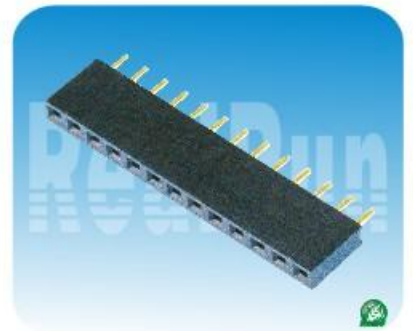
02.5系列: 2.54mm单排母,180度,U形端子 Spec:2.54mm Female Header,Single Row,Straight Positions:1*2~1*40 Plastics Height:7.1mm
