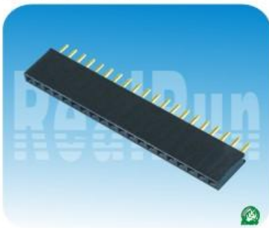
02.5系列: 2.54mm单排母,180度 Spec:2.54mm Female Header,Single Row,Straight Positions:1*2~1*40 Plastics Height:8.5mm Y-Type Terminal
