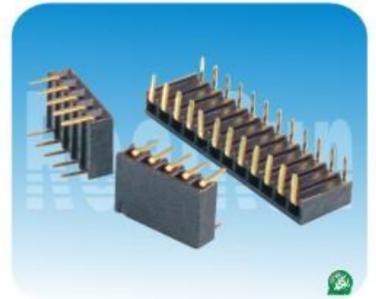
02.5 系列: 2.54mm单排母,90度,侧插型 Spec:2.54mm Female Header,Single Row, Side Entry,Right Angle Positions:1*2~1*40 Plastics Height:3.4mm
