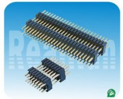
01.3系列: 1.27*2.54mm双排针,双塑,180度 Spec:1.27 mm Board Spacer,Dual Row, Dual Plastics Straight Positions:2*2~2*50 Plastics Height:1.7/2.54mm
