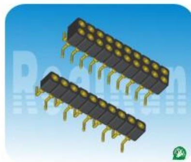
02.A系列:2.0mm 圆孔 单/双排 SMT Spec:2.0mm Pitch Machine Pin Socket Single/Dual Row SMT Plastics Height:2.8 Positions:1*2~1*40/2*2~2*40
