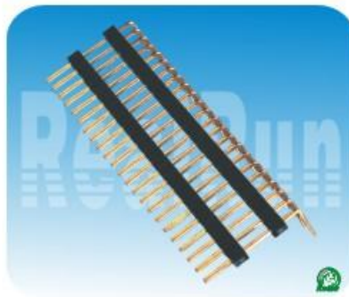
01.4 系列: 2.0mm单排针,双塑,90度 TYPE 1 Spec:2.0mm Dual Plastics,Single Row,Right Angle,Type 1 Positions:1*2~1*40 Plastics Height:2.0mm
